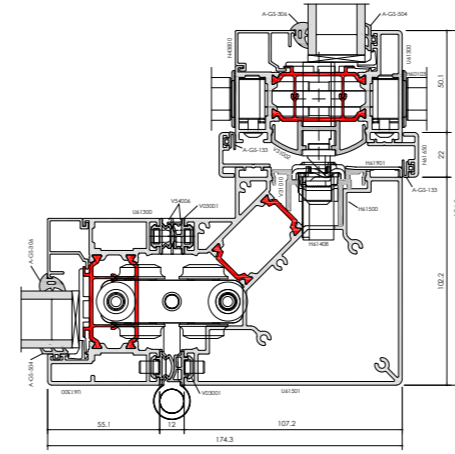
F82 FLOATING CORNER POST / C1
