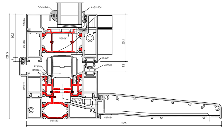
F82 HEAD WITH 40MM ADDON FOR TRICKLE VENT / A1
