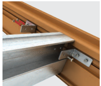
Fix rafters to ringbeam
