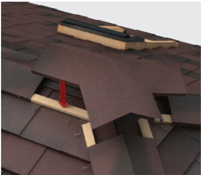
Fix rafter cap and ridge
